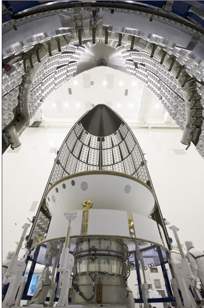
The Mars Science Laboratory inside the fairing that is being installed around it.
