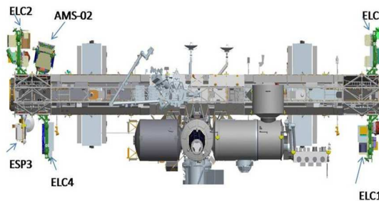
ISS truss configuration with ELC3 and AMS-02
