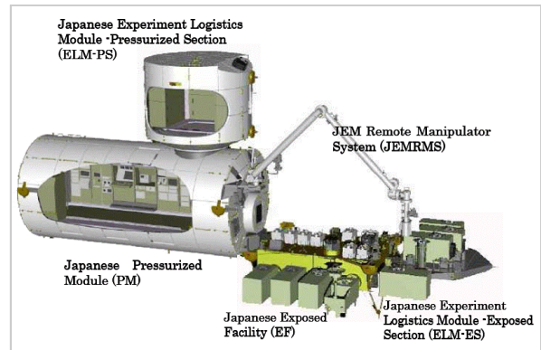
Figure 2: Kibo and its components
