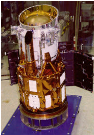
The Assembled WIRE Spacecraft
