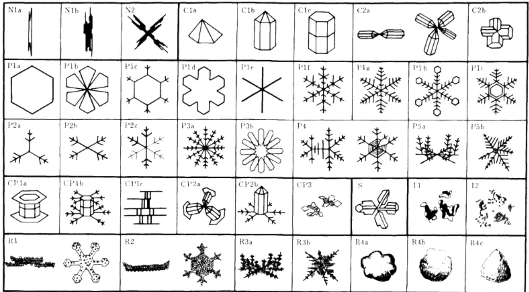
FIG. 197. General classification of snow crystals, sketches.
