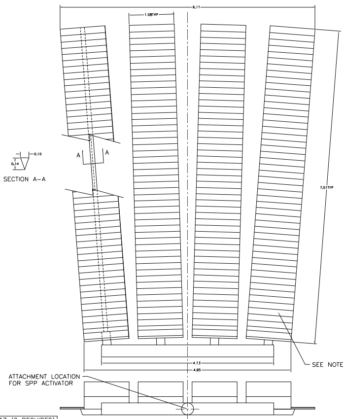
ITEM #17 (2 REQUIRED) SPP PV ARRAYS
