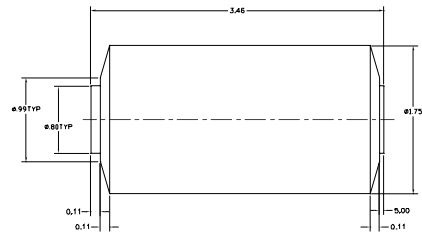
ITEM #9 (2 REQUIRED) U.S. HAB & LAB MODULE
