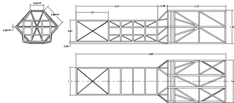
ITEM #31 (2 REQUIRED) S-3/4, P-3/4 TRUSS
