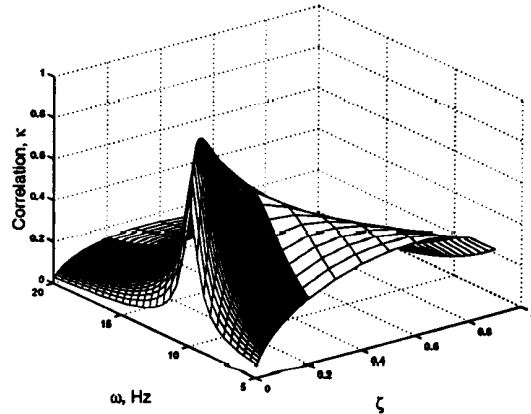
Figure 3: Surface Map of Correlation Coefficient \kappa_\gamma Obtained from Correlation Filtering of the Test Signal with a Subset of the Laplace Wavelet Dictionary \Psi at \tau = t_o = 0 s
