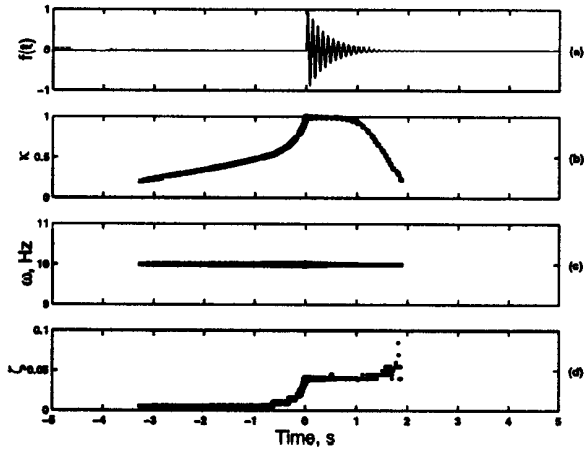
Figure 2: Correlation Filtering of the Test Signal with the Laplace Wavelet Dictionary \Psi : Test Signal f(t) (a), Peak Correlation Coefficient \kappa(\tau) (b), Wavelet Frequency \bar{\omega} Associated with Peak \kappa (c), Wavelet Damping \bar{\zeta} Associated with Peak \kappa (d)
