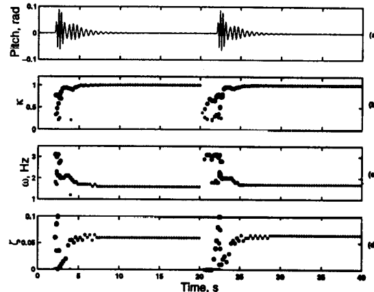
Figure 9: Correlation Filtering of the Nonlinear Simulation Response with the Laplace Wavelet Dictionary \Psi : Pitch State Variable (a), Correlation Coefficient \kappa (b), Wavelet Frequency \bar{\omega} Associated with Peaks of \kappa (c), Wavelet Damping \bar{\zeta} Associated with Peaks of \kappa (d)
