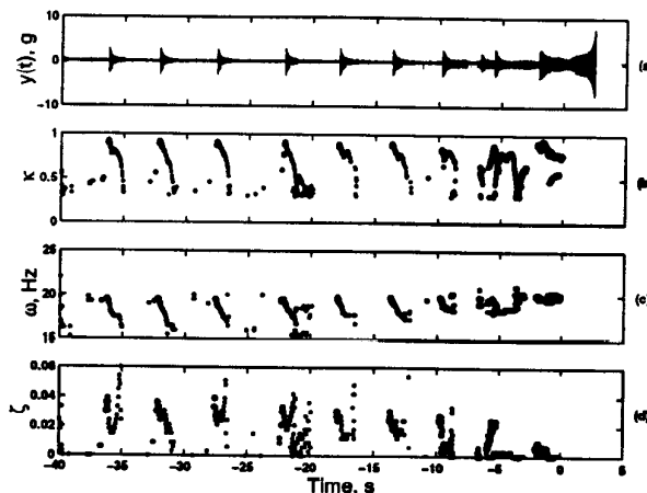
Figure 5: Correlation Filtering of the DAST Data with the Laplace Wavelet Dictionary: Left Wingtip Acceleration (a), Peak Correlation Values \kappa(\tau) > 0.3 (b), Wavelet Frequencies Associated with Peak Correlations (c), Corresponding Wavelet Damping Values (d)
