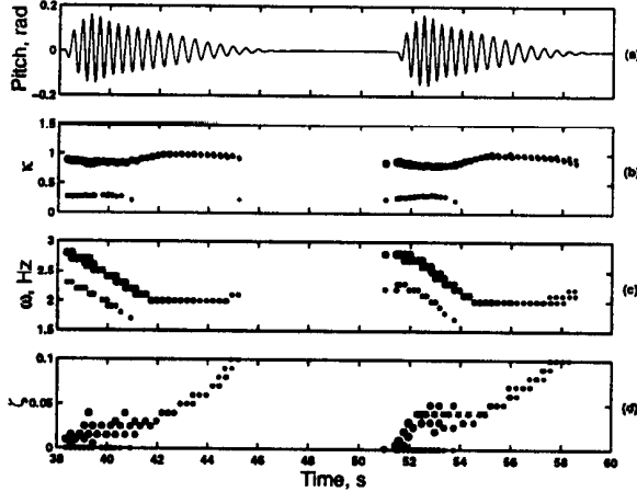
Figure 10: Correlation Filtering of the Texas A&M University Nonlinear Testbed with the Laplace Wavelet Dictionary \Psi : Pitch Measurement (a), Correlation Coefficient \kappa (b), Wavelet Frequency \bar{\omega} Associated with Peaks of \kappa (c), Wavelet Damping \bar{\zeta} Associated with Peaks of \kappa (d)
