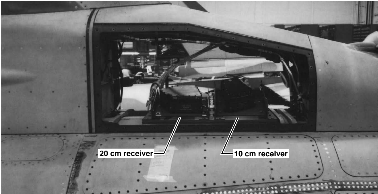
Fig. 5 Receiver bay.
