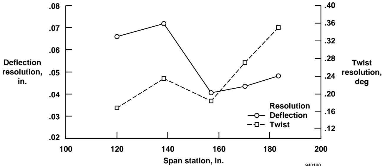
Fig. 7 F-16 FDMS deflection and twist resolution.
