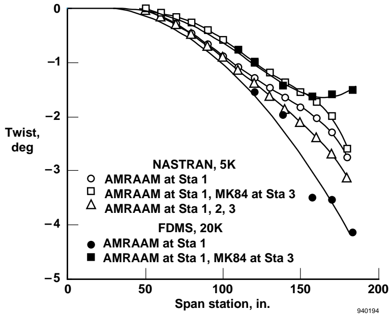
Fig. 20 Stores variation effect, 0.9M, 5g.
