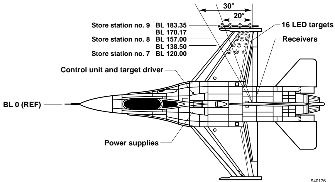
Fig. 3 FDMS installation.
