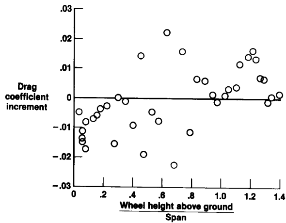
Fig. 6 Ground-effect drag coefficient increment; CID/720 at 40° flap.
