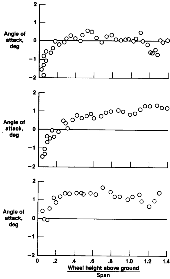
Fig. 5 Angle-of-attack profiles during various approaches.
