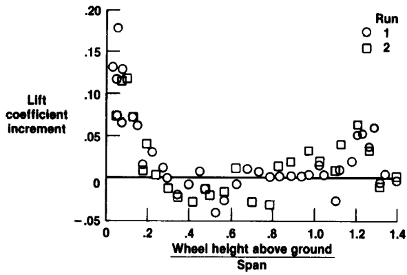
Fig. 4 Ground-effect lift coefficient increment; CID/720 at 40° flap.
