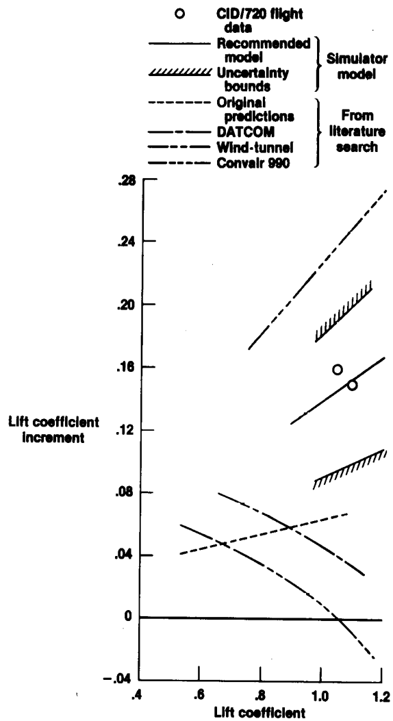
Fig. 8 Ground-effect lift coefficient increment at ground level, 40° flap.
