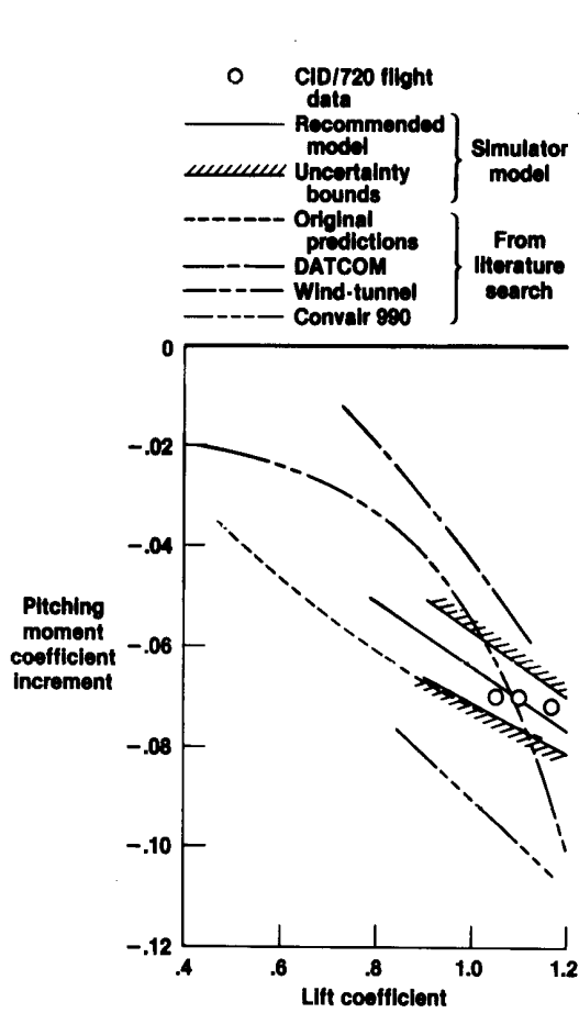
Fig. 7 Ground-effect pitching moment coefficient increment at ground level, 40° flap.
