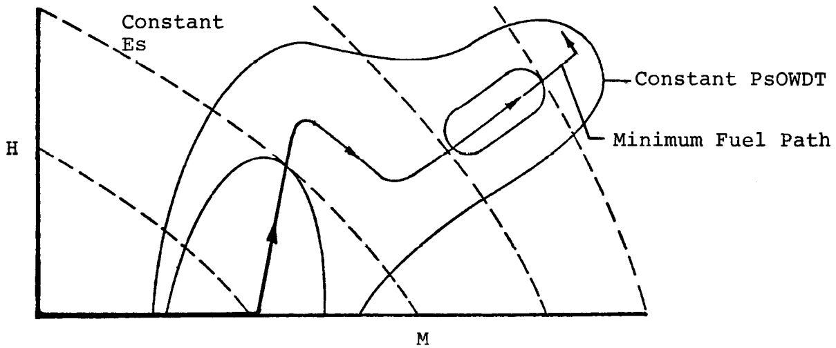
Figure 10. Minimum fuel path on plot of PsOWDT and constant energy
