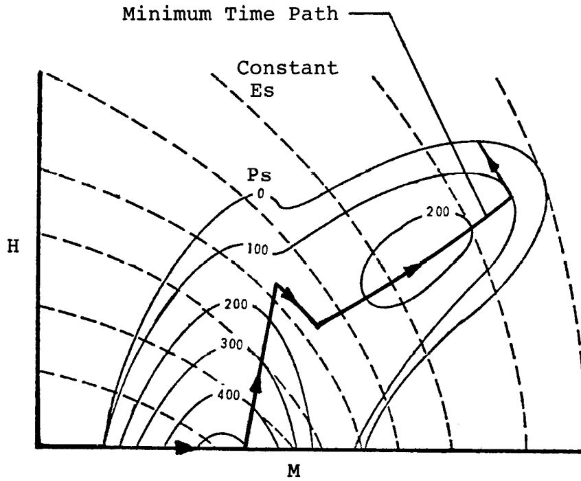
Figure 9. Minimum time path on plot of Ps and constant energy
