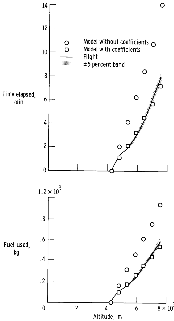
(a) 26° wing sweep angle.
