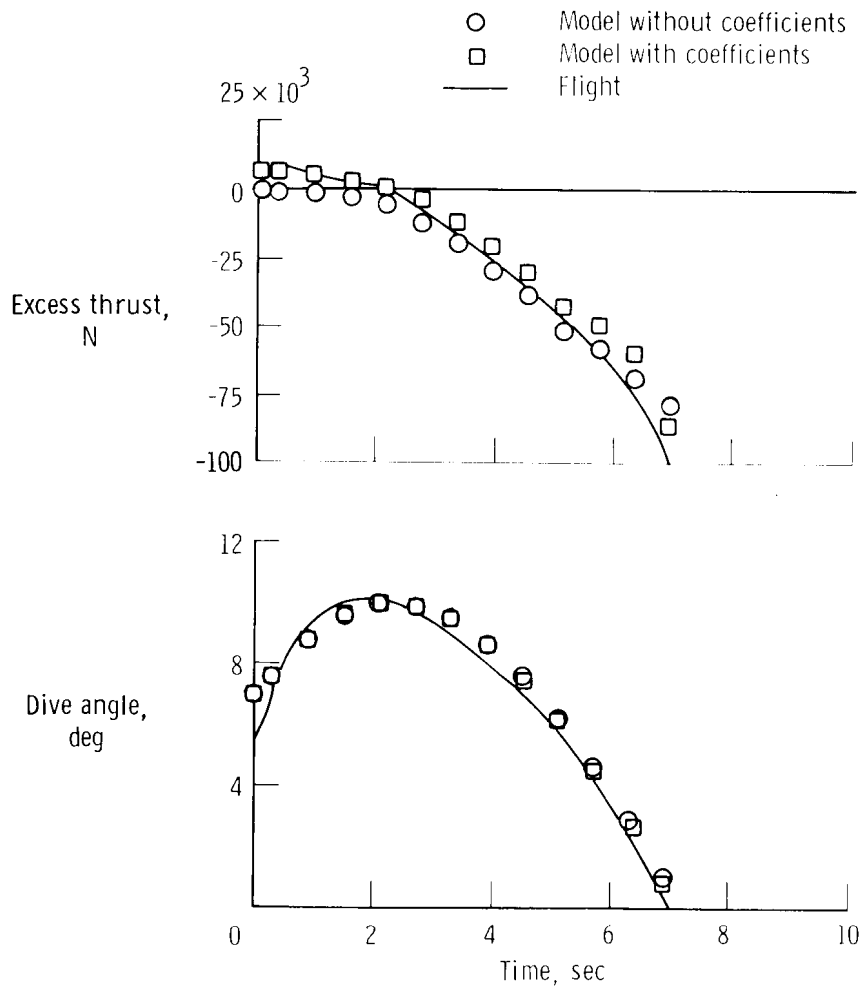
(a) Pushover pullup.
