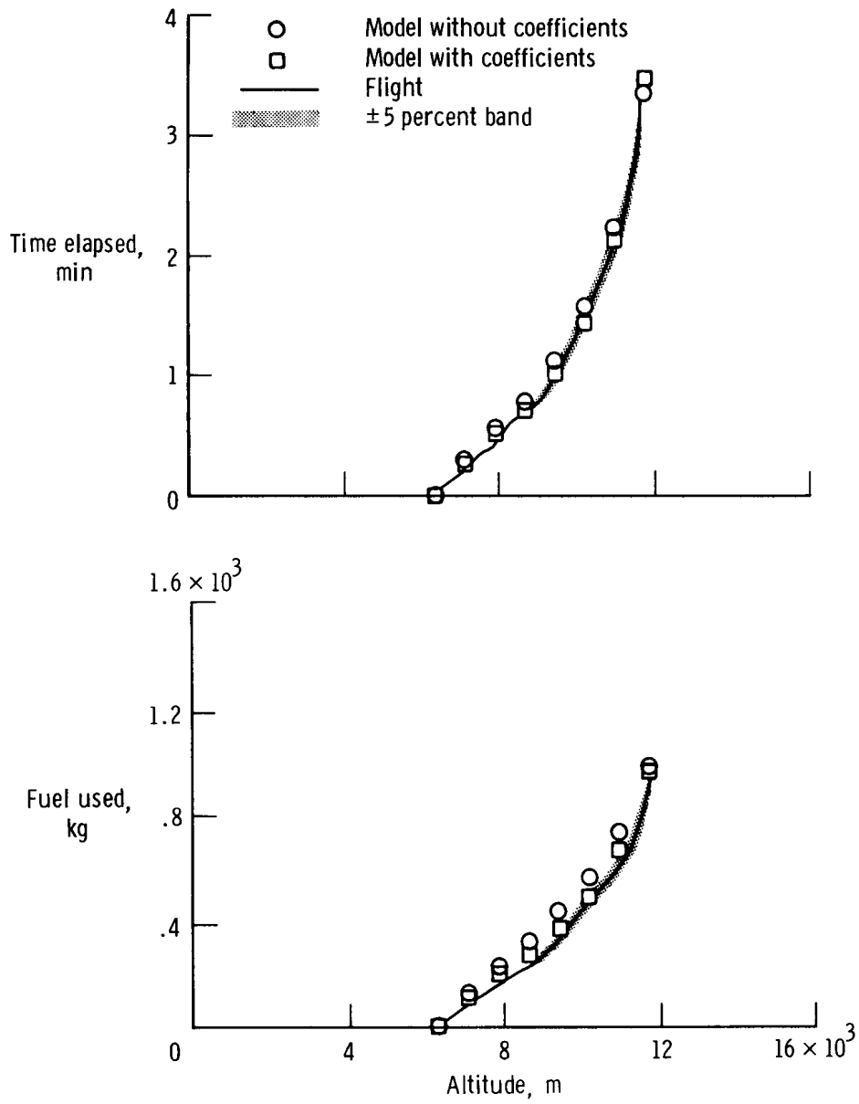
(b) 36° wing sweep angle.
