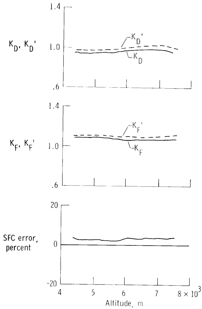
Figure 9. Modeling coefficients and SFC error for a typical subsonic constant-Mach-number climb. 26° wing sweep angle, intermediate power.
