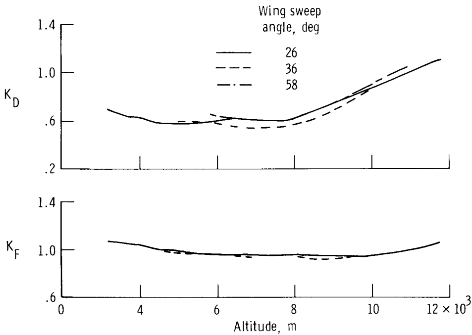
Figure 3. Modeling coefficient correlation for subsonic constant-Mach-number climbs and level accelerations. Maximum afterburning power.
