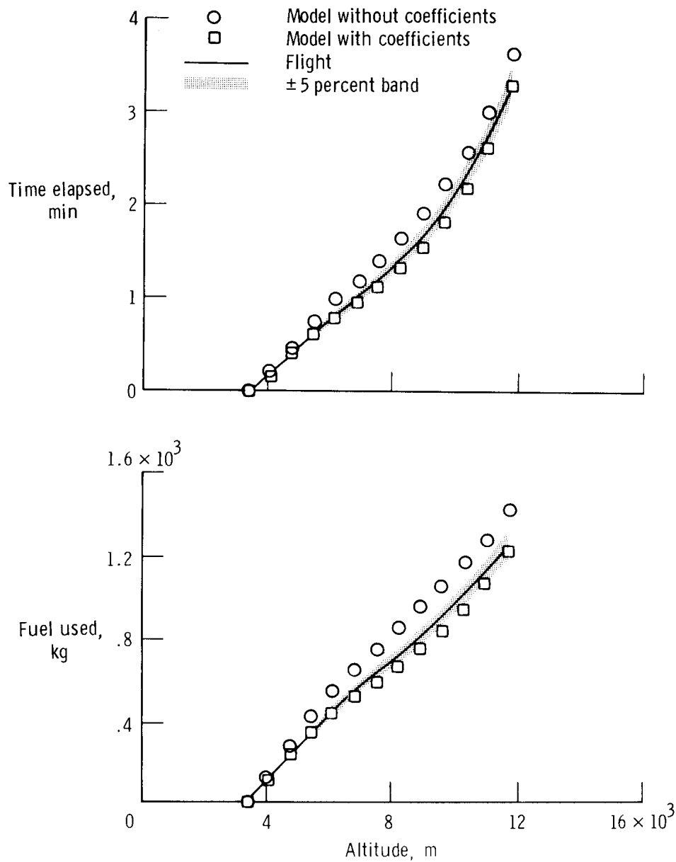
(a) 26° wing sweep angle.
