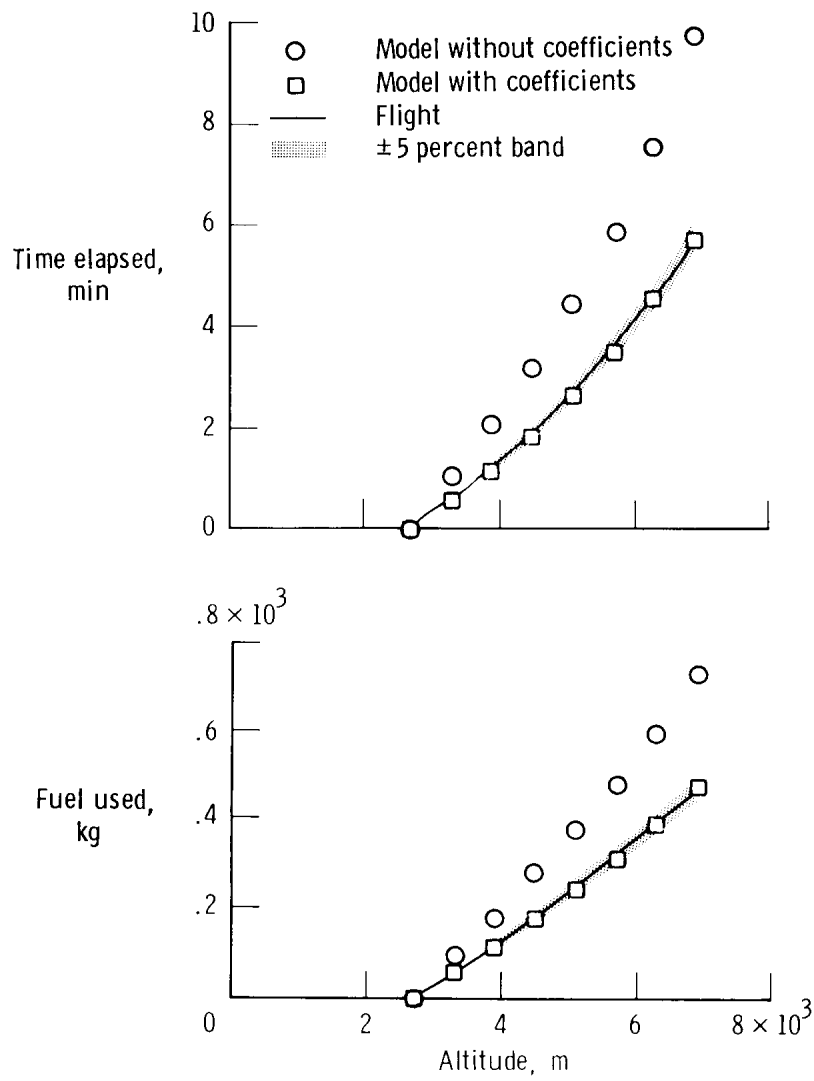
(c) 58° wing sweep angle.
