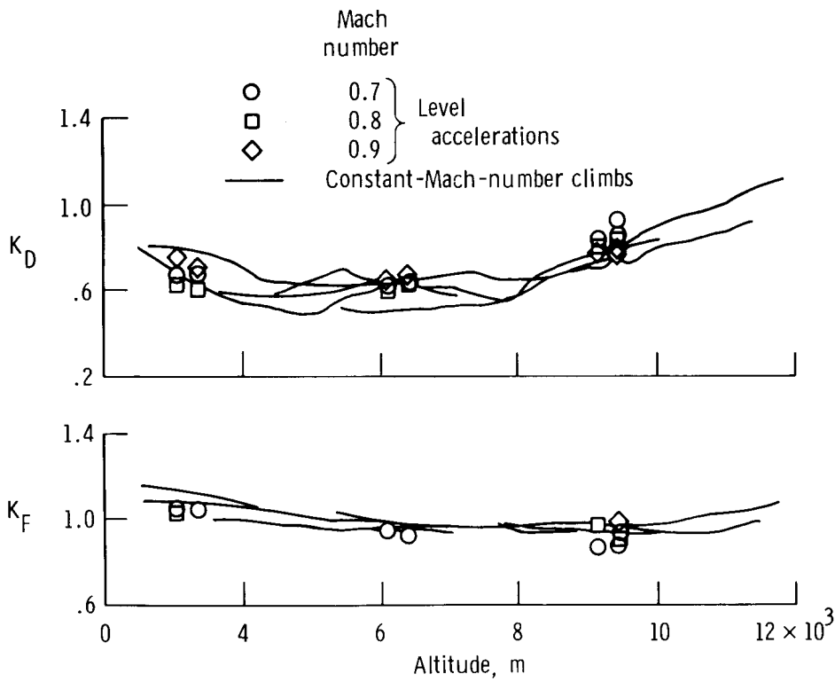
Figure 2. Modeling coefficients for subsonic constant-Mach-number climbs and level accelerations. 26^\circ wing sweep angle, maximum afterburning power.
