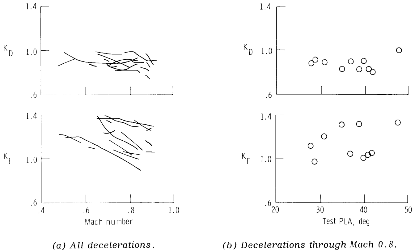
Figure 10. Modeling coefficients for level decelerations at power settings below intermediate. All wing sweep angles.
