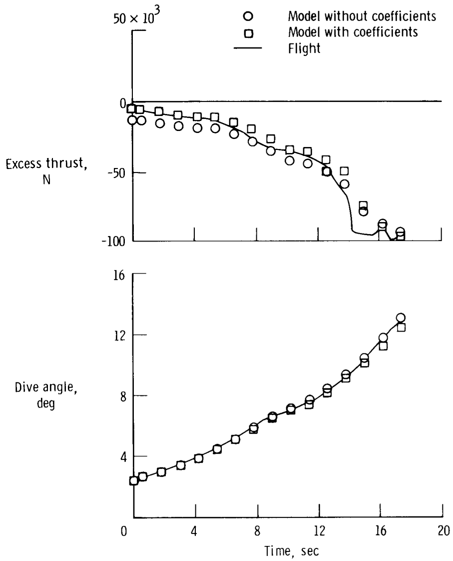
(b) Windup turn.
