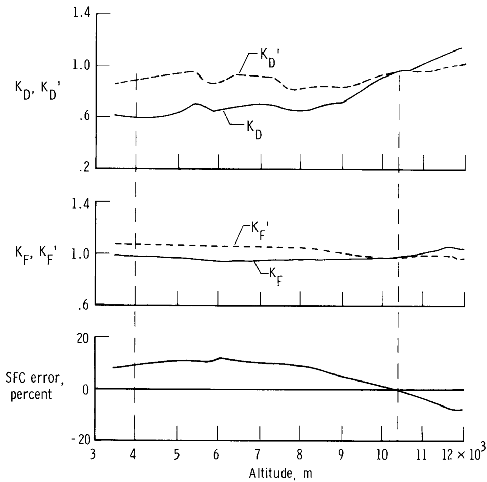
Figure 5. Modeling coefficients and SFC error for a typical subsonic constant-Mach-number climb. 26° wing sweep angle, maximum afterburning power.
