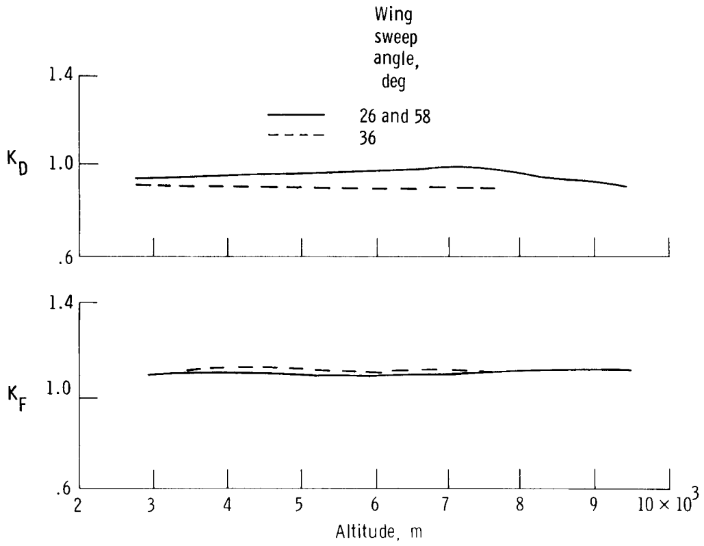
Figure 7. Modeling coefficient correlation for subsonic constant-Mach-number climbs and level accelerations. Intermediate power.
