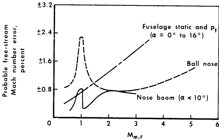
Figure 9.— Probable free-stream Mach number error for three X-15 air-data systems.
