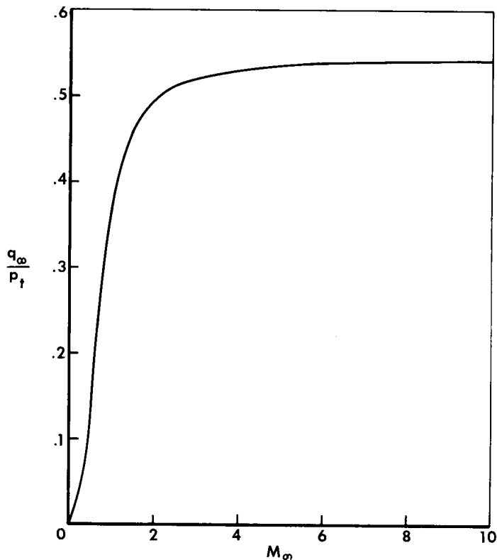
Figure 5.— Ratio of free-stream dynamic pressure to ball-nose stagnation pressure for speeds up to M_\infty = 10 .
