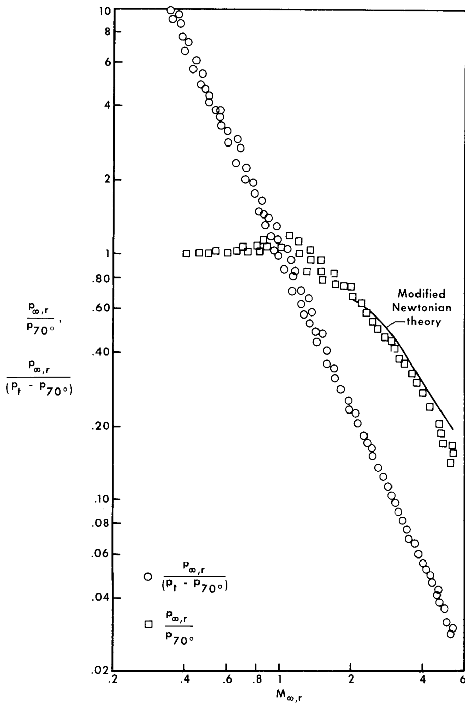
Figure 10.— Free-stream static pressure calibration.
