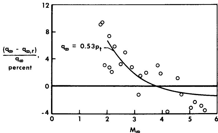
Figure 13.— Dynamic-pressure error using q_\infty = 0.53p_t .
