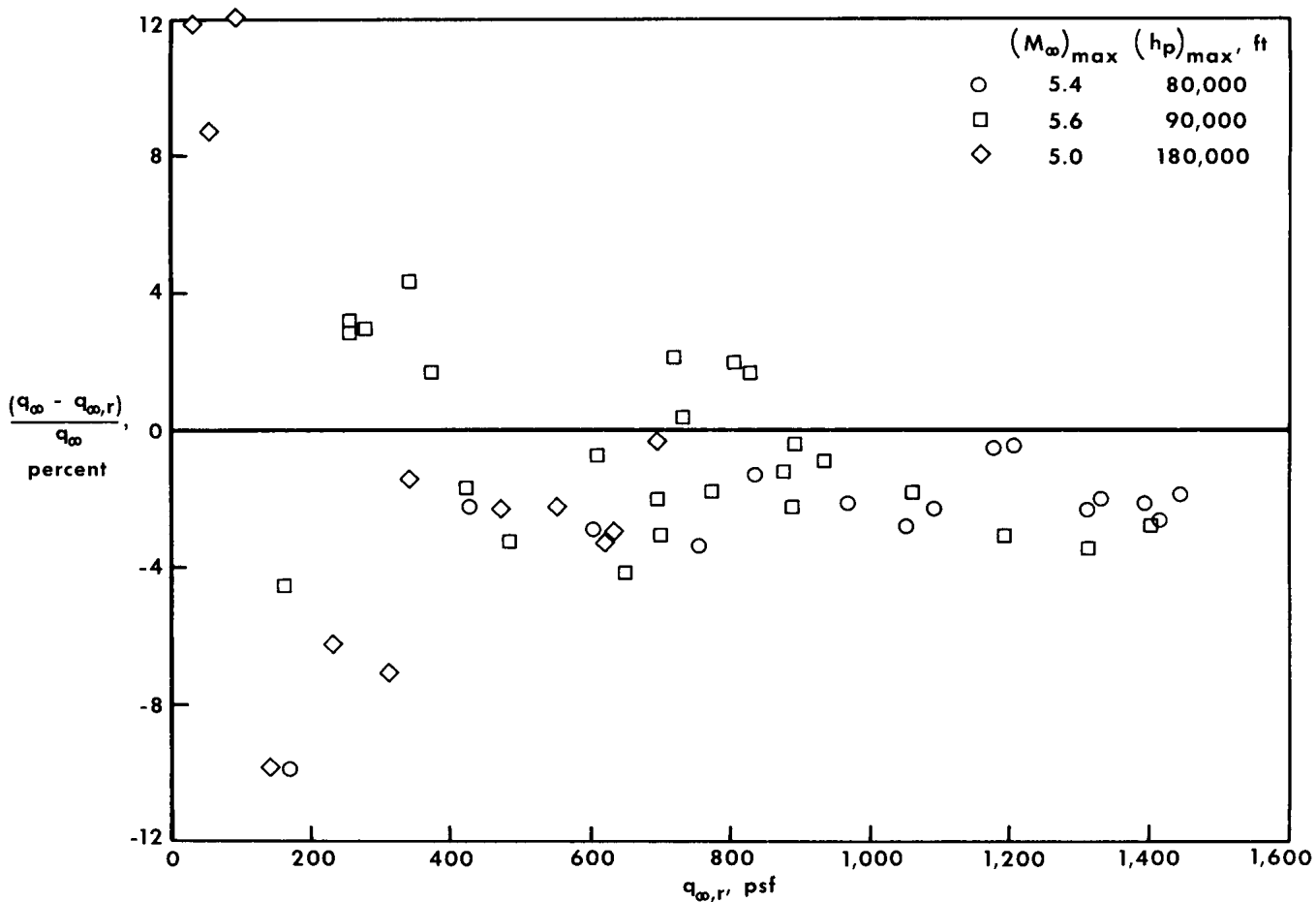
Figure 12.— Percent difference between ball-nose and reference dynamic pressures.
