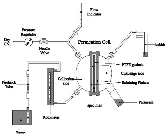
Permeation system configured for ambient pressure permeation of liquid propellant
